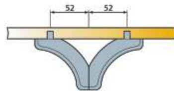
Back-to-back application
